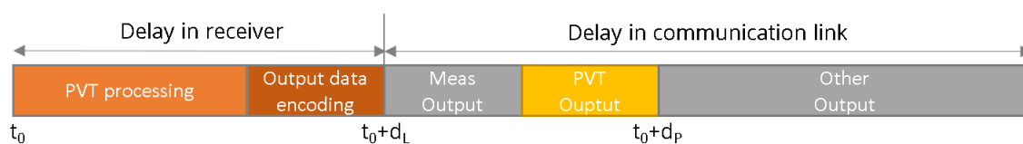
Figure 2-3: PVT latency.
